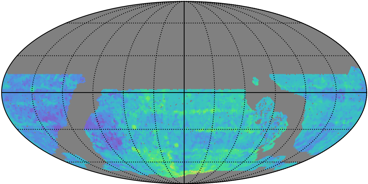
roll_uniform_early_half_mjdp253_v3.4_10yrs WFD y band: Median Season Length
