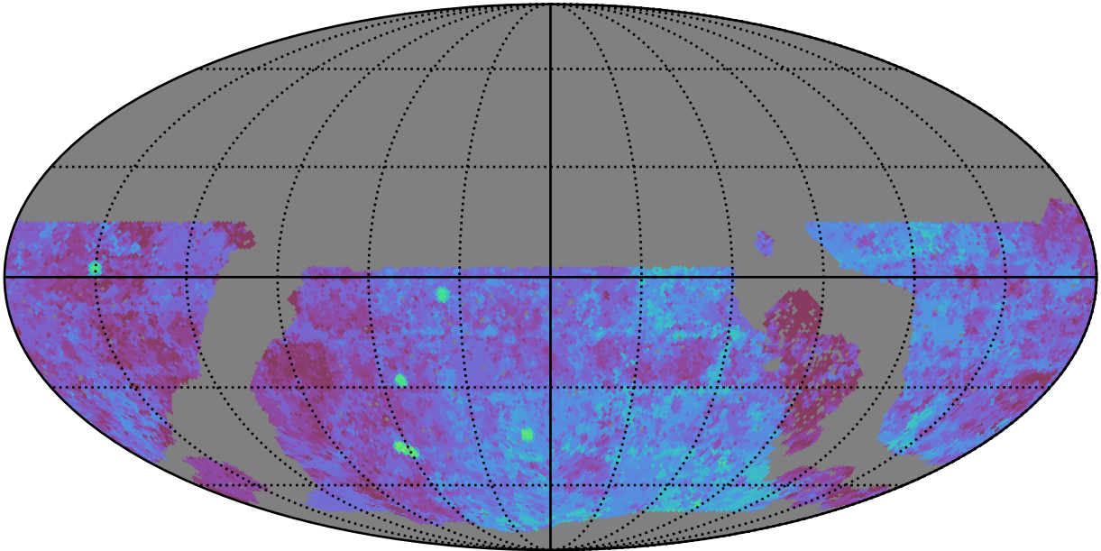
roll_uniform_early_half_mjdp253_v3.4_10yrs WFD u band: Median Season Length
