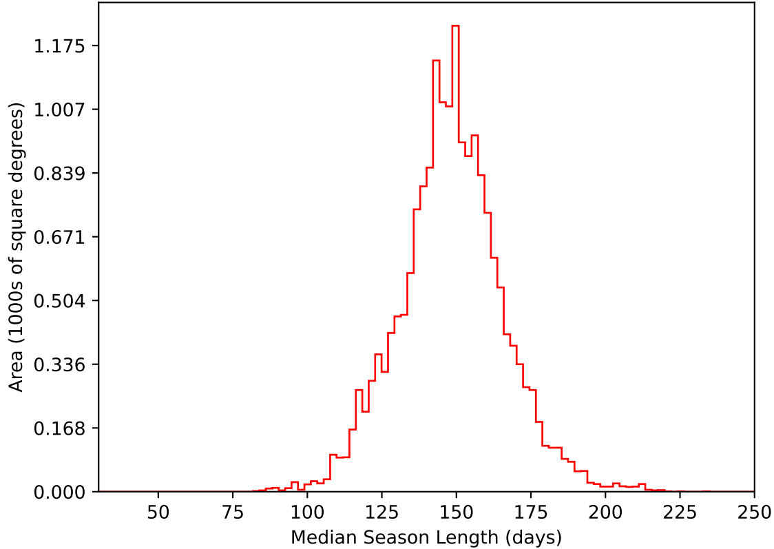
roll_uniform_early_half_mjdp253_v3.4_10yrs WFD i band: Median Season Length
