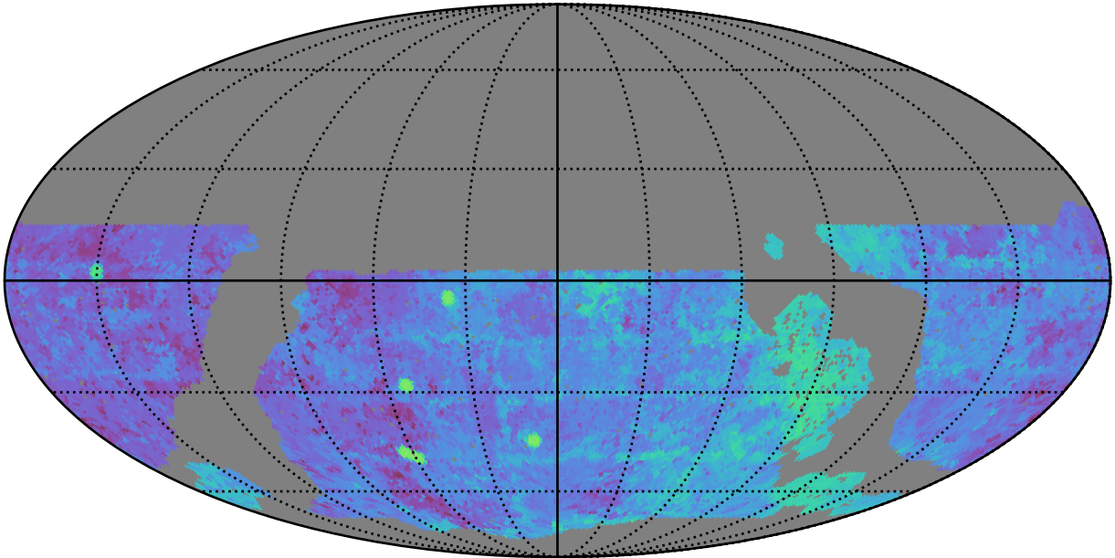
roll_uniform_early_half_mjdp253_v3.4_10yrs WFD g band: Median Season Length
