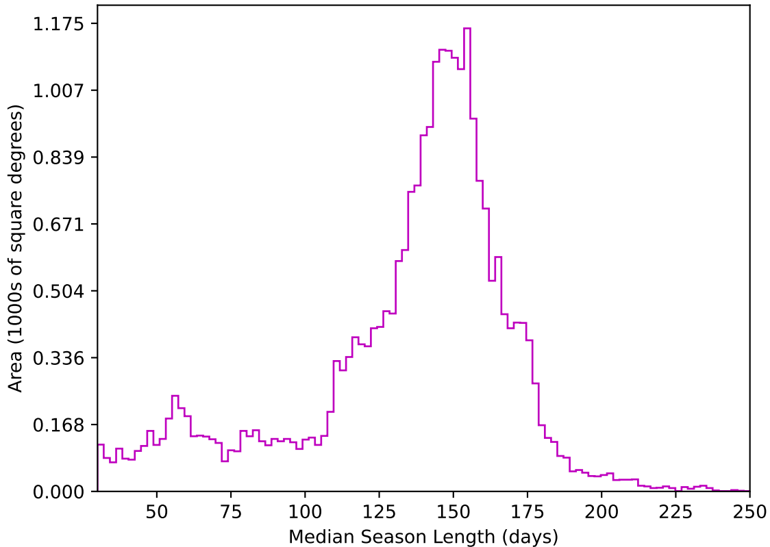
roll_uniform_early_half_mjdp253_v3.4_10yrs All sky z band: Median Season Length
