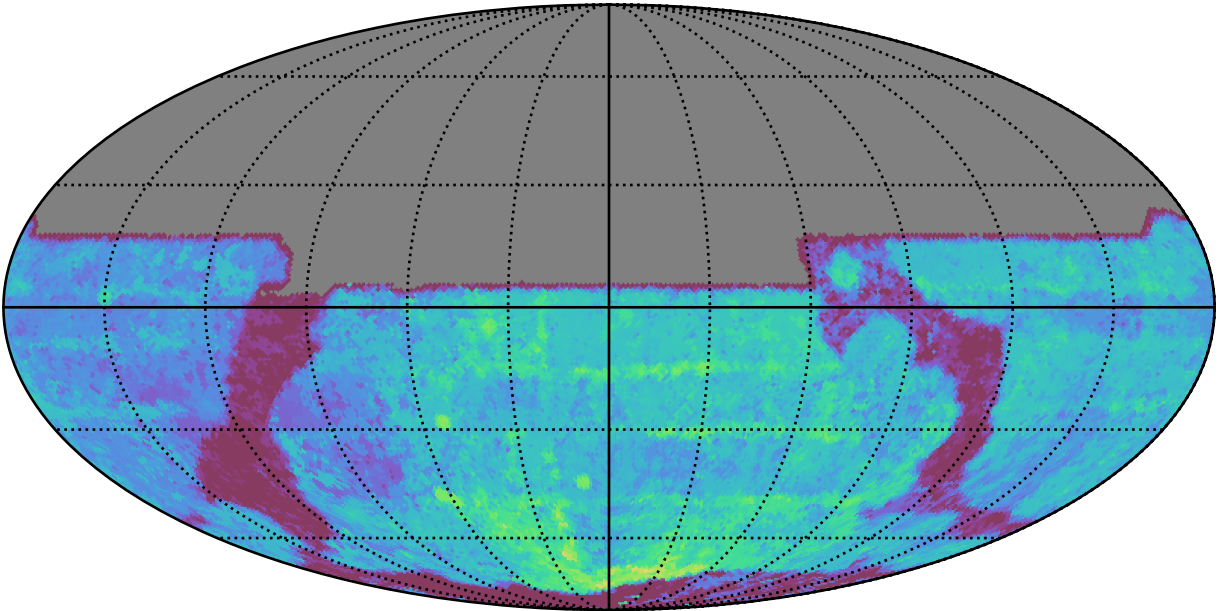
roll_uniform_early_half_mjdp253_v3.4_10yrs All sky y band: Median Season Length
