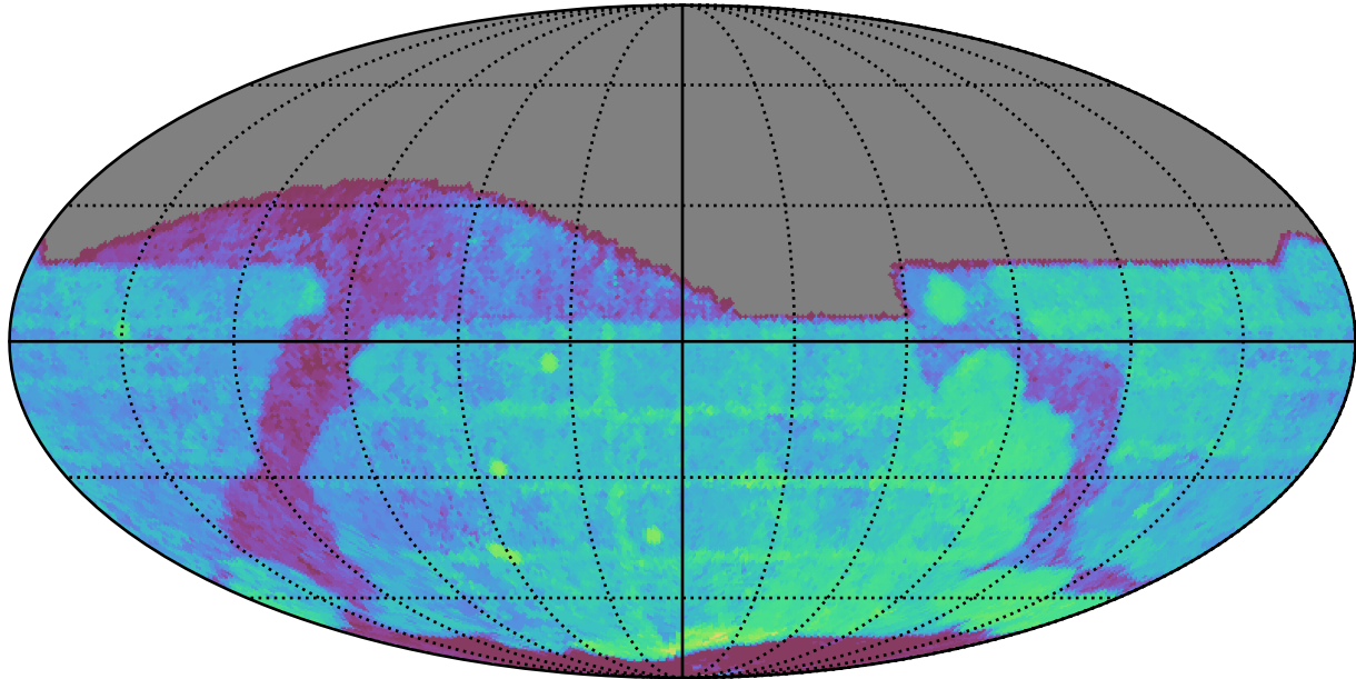
roll_uniform_early_half_mjdp253_v3.4_10yrs All sky r band: Median Season Length
