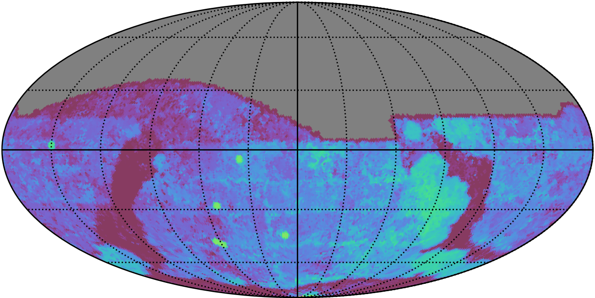
roll_uniform_early_half_mjdp253_v3.4_10yrs All sky g band: Median Season Length
