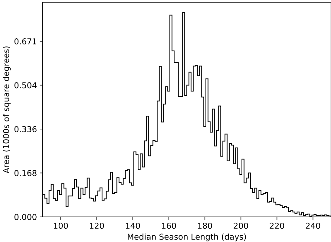
roll_uniform_early_half_mjdp253_v3.4_10yrs All sky all bands: Median Season Length
