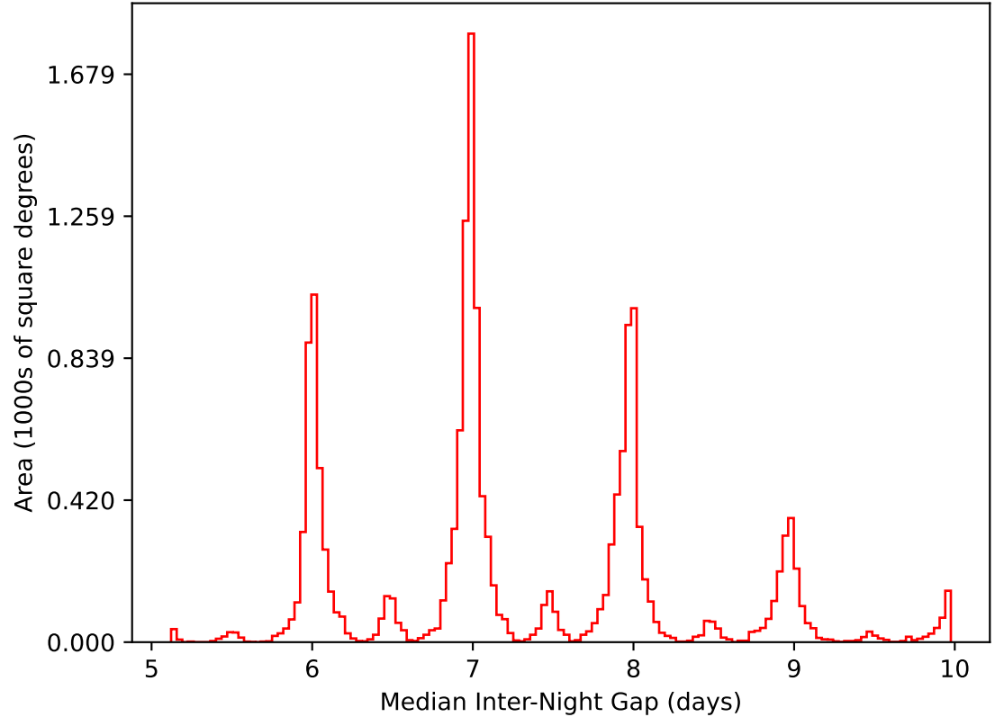
roll_uniform_early_half_mjdp253_v3.4_10yrs WFD i band: Median Inter-Night Gap
