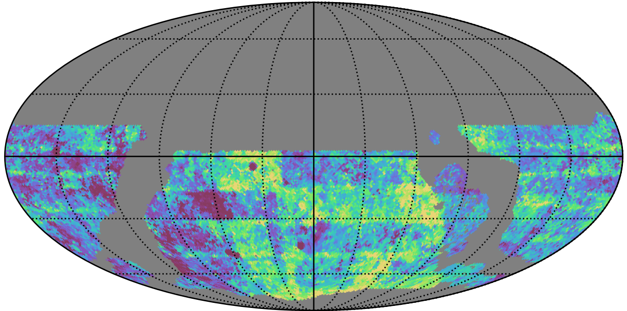
roll_uniform_early_half_mjdp253_v3.4_10yrs WFD g band: Median Inter-Night Gap
