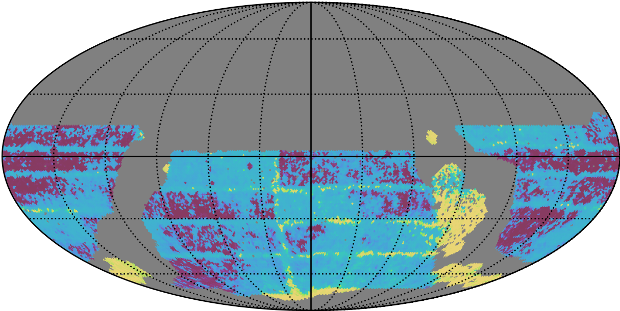
roll_uniform_early_half_mjdp253_v3.4_10yrs WFD all bands: Median Inter-Night Gap
