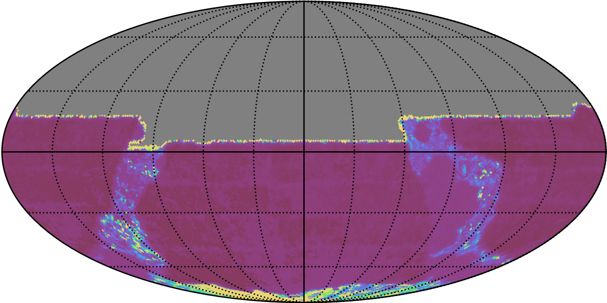
roll_uniform_early_half_mjdp253_v3.4_10yrs All sky y band: Median Inter-Night Gap
