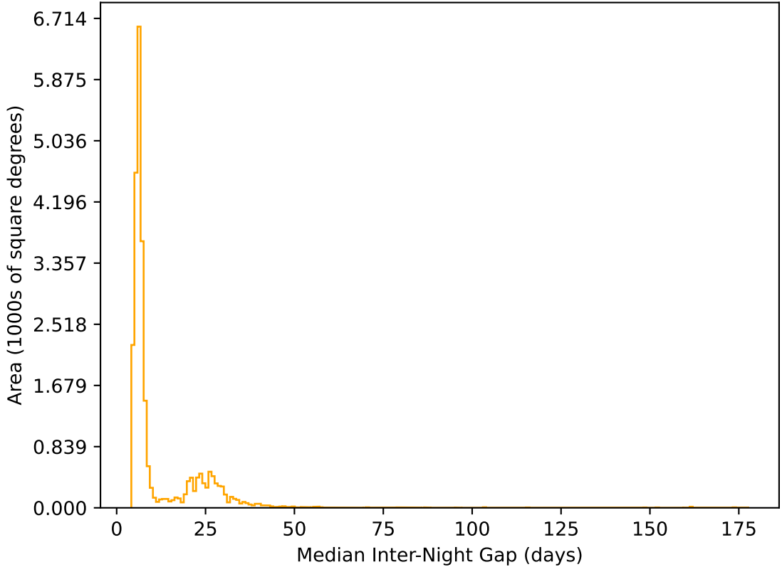
roll_uniform_early_half_mjdp253_v3.4_10yrs All sky r band: Median Inter-Night Gap
