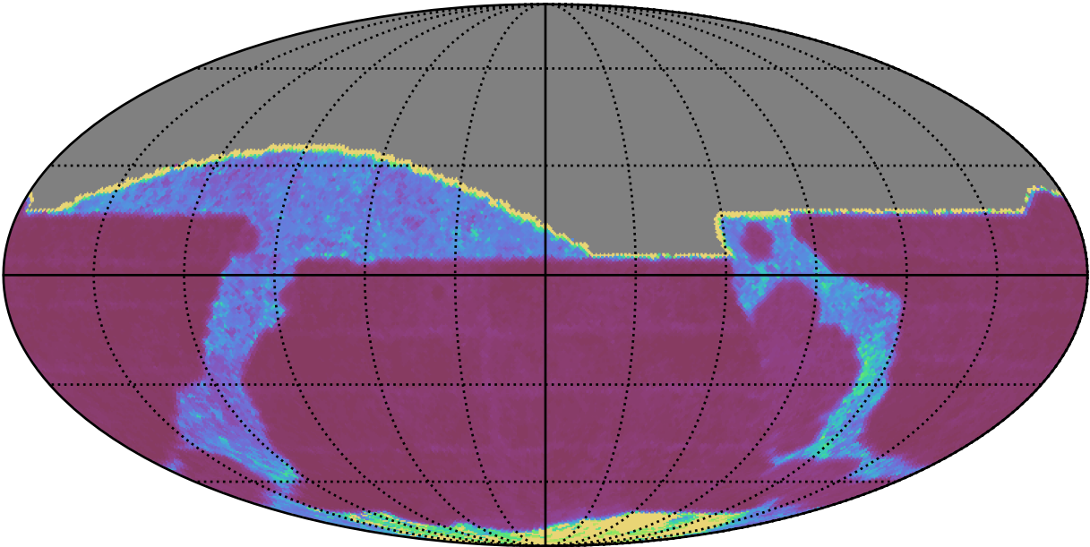
roll_uniform_early_half_mjdp253_v3.4_10yrs All sky i band: Median Inter-Night Gap
