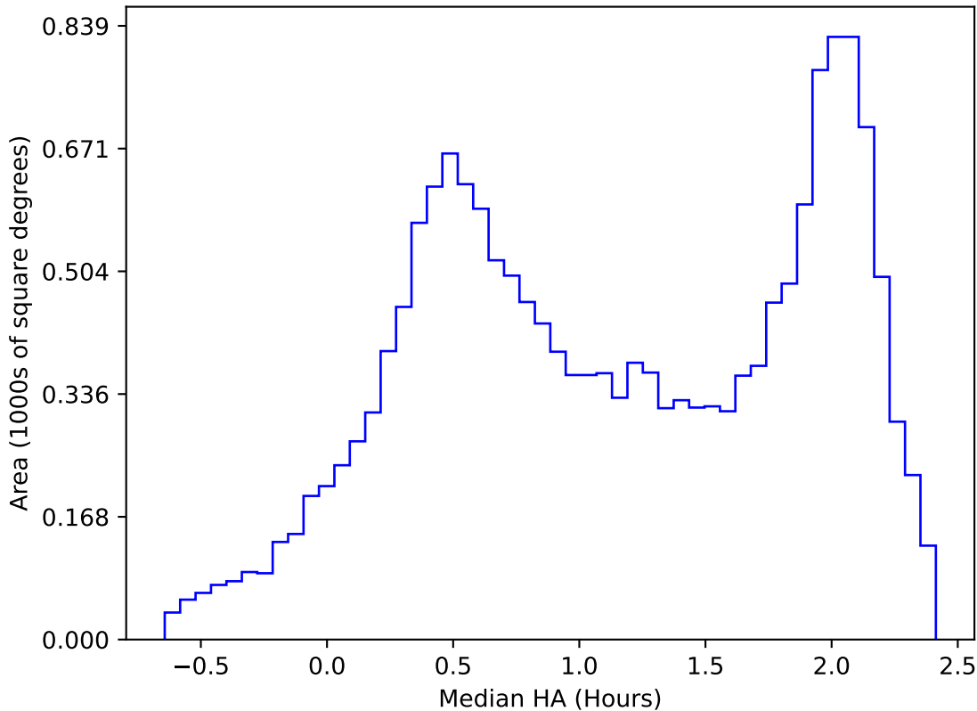
roll_uniform_early_half_mjdp253_v3.4_10yrs WFD y band: Median HA
