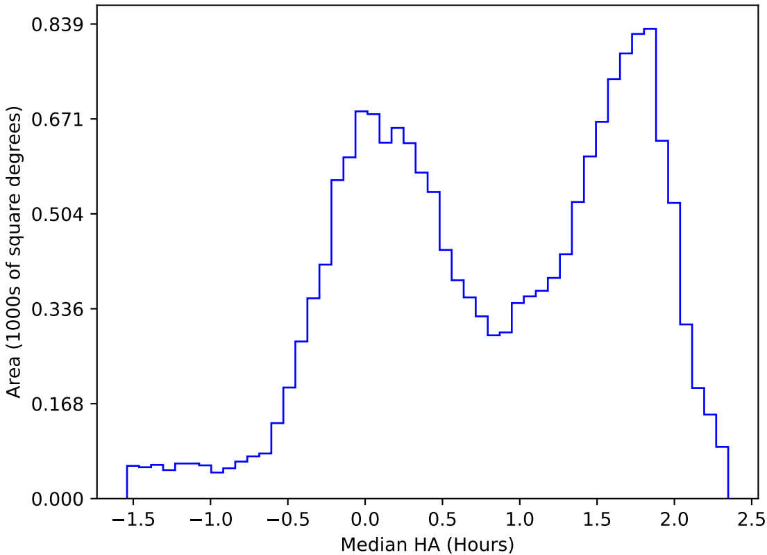
roll_uniform_early_half_mjdp253_v3.4_10yrs WFD u band: Median HA
