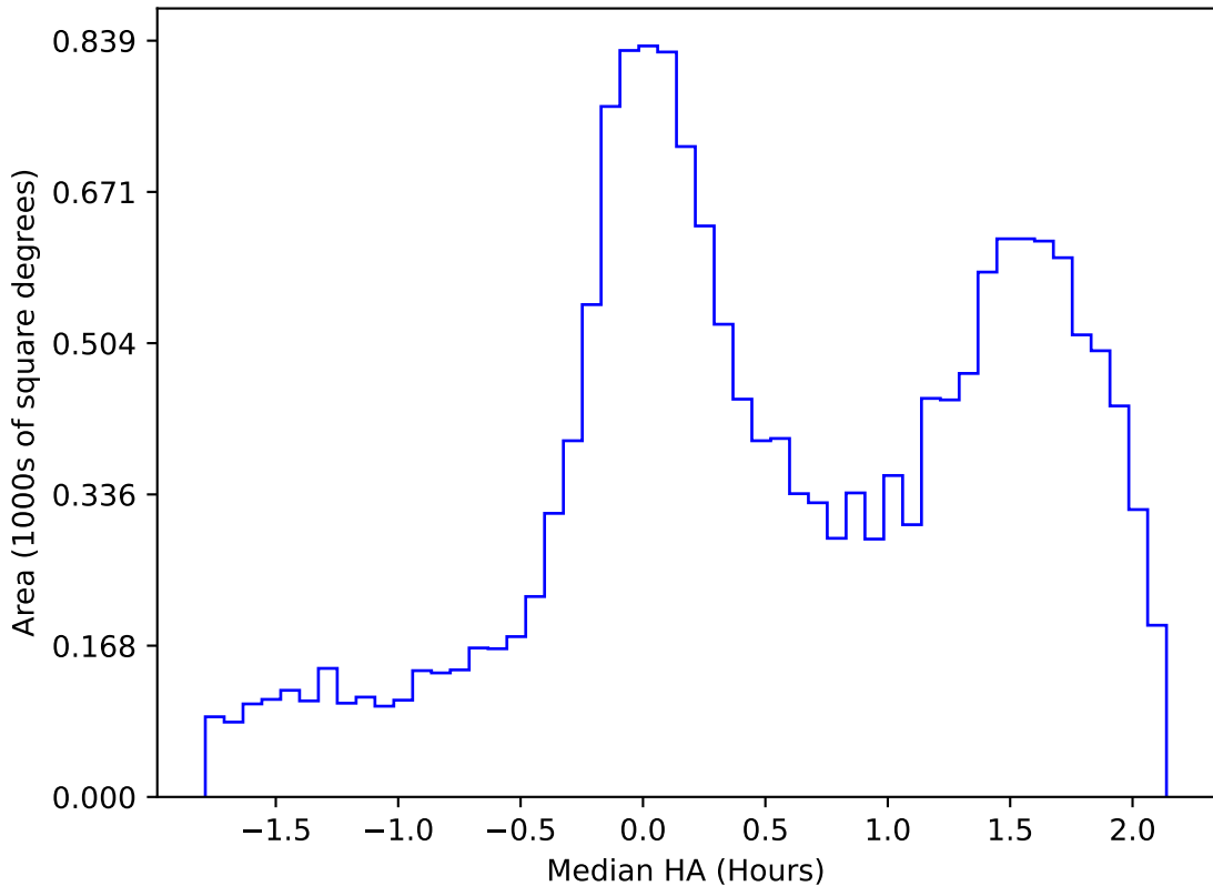
roll_uniform_early_half_mjdp253_v3.4_10yrs WFD g band: Median HA
