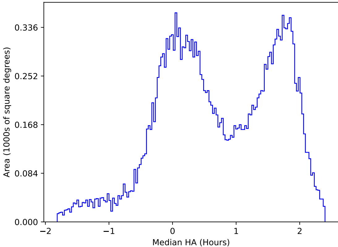
roll_uniform_early_half_mjdp253_v3.4_10yrs All sky u band: Median HA
