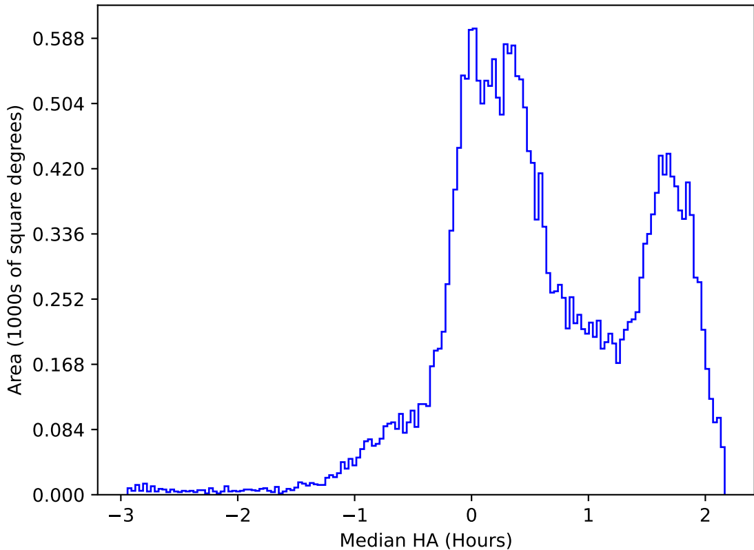
roll_uniform_early_half_mjdp253_v3.4_10yrs All sky r band: Median HA
