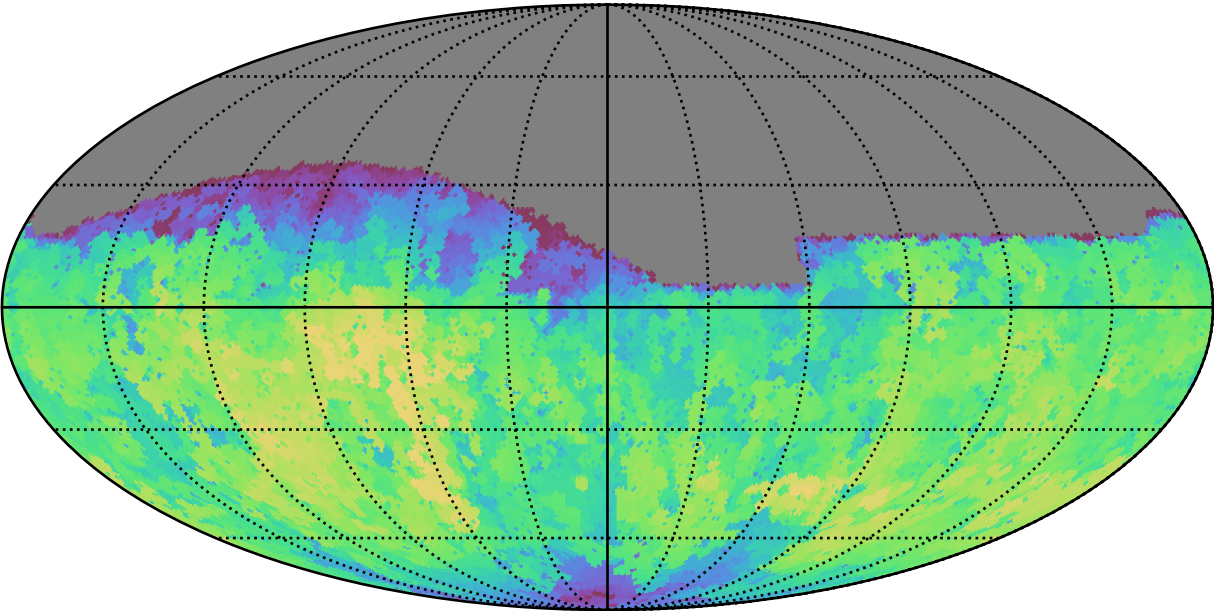
roll_uniform_early_half_mjdp253_v3.4_10yrs Yr 1 all bands: Max fiveSigmaDepth
