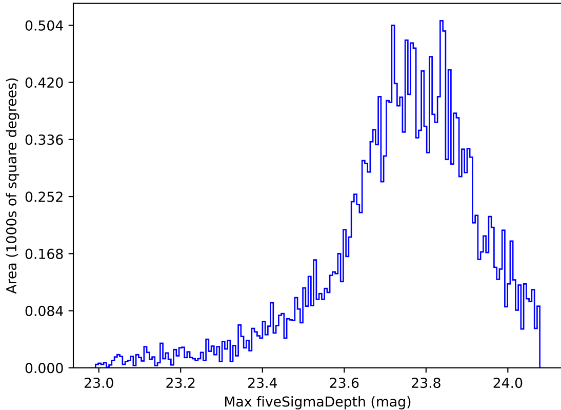
roll_uniform_early_half_mjdp253_v3.4_10yrs All sky u band: Max fiveSigmaDepth
