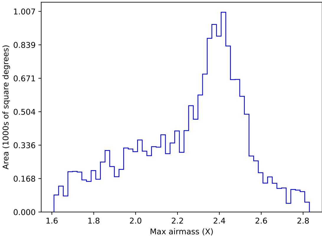
roll_uniform_early_half_mjdp253_v3.4_10yrs WFD r band: Max airmass
