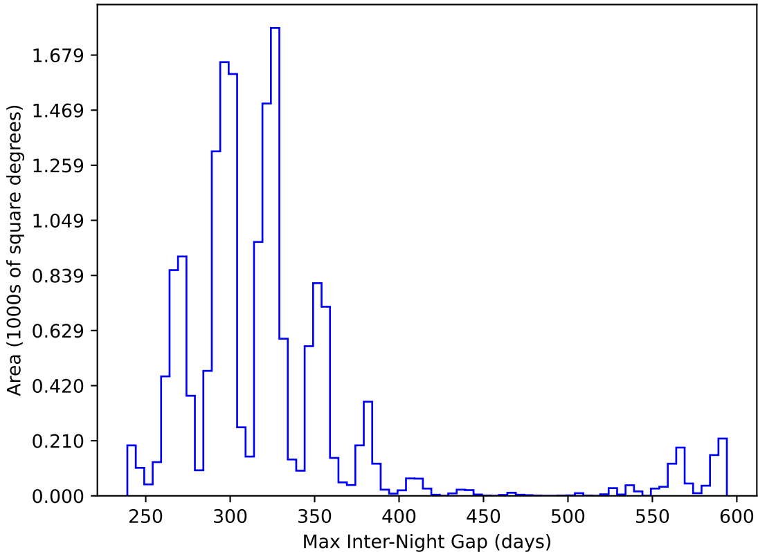
roll_uniform_early_half_mjdp253_v3.4_10yrs WFD y band: Max Inter-Night Gap
