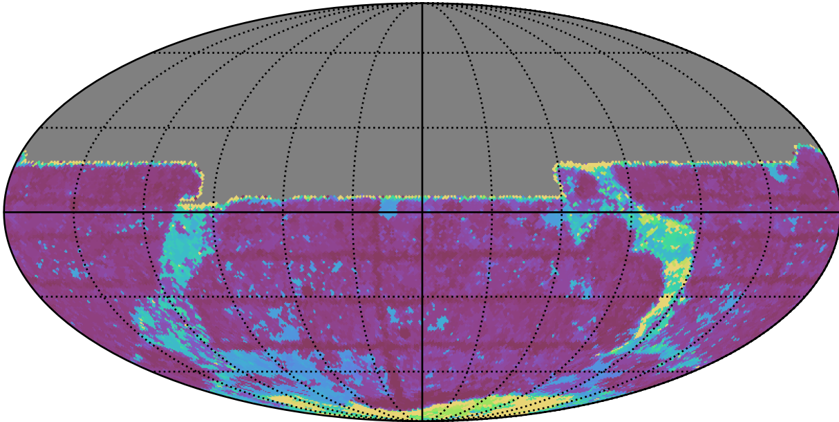
roll_uniform_early_half_mjdp253_v3.4_10yrs All sky y band: Max Inter-Night Gap
