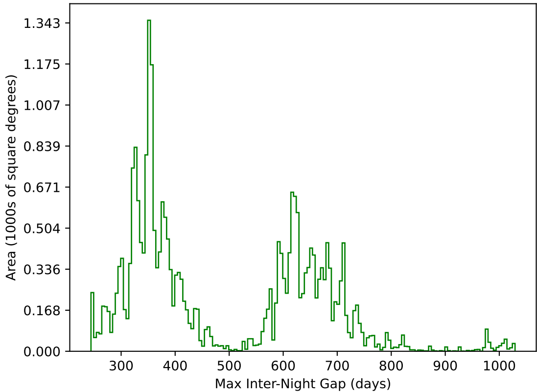
roll_uniform_early_half_mjdp253_v3.4_10yrs All sky g band: Max Inter-Night Gap
