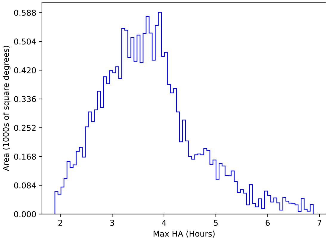
roll_uniform_early_half_mjdp253_v3.4_10yrs WFD u band: Max HA
