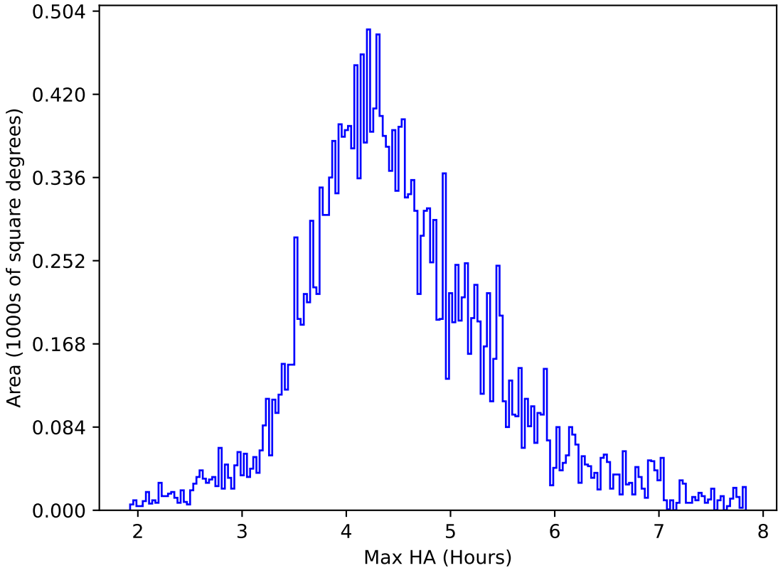
roll_uniform_early_half_mjdp253_v3.4_10yrs All sky y band: Max HA
