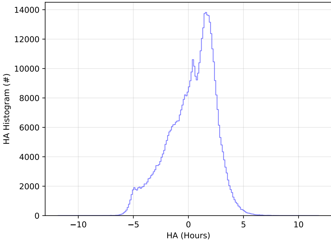
roll_uniform_early_half_mjdp253_v3.4_10yrs WFD r band: HA Histogram
