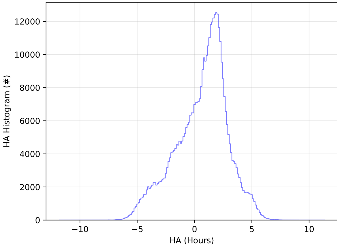
roll_uniform_early_half_mjdp253_v3.4_10yrs All sky z band: HA Histogram
