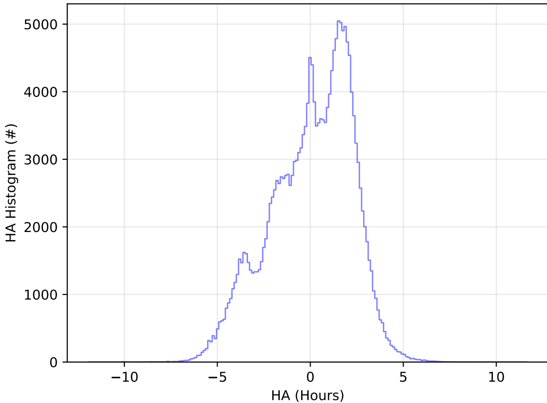
roll_uniform_early_half_mjdp253_v3.4_10yrs All sky g band: HA Histogram
