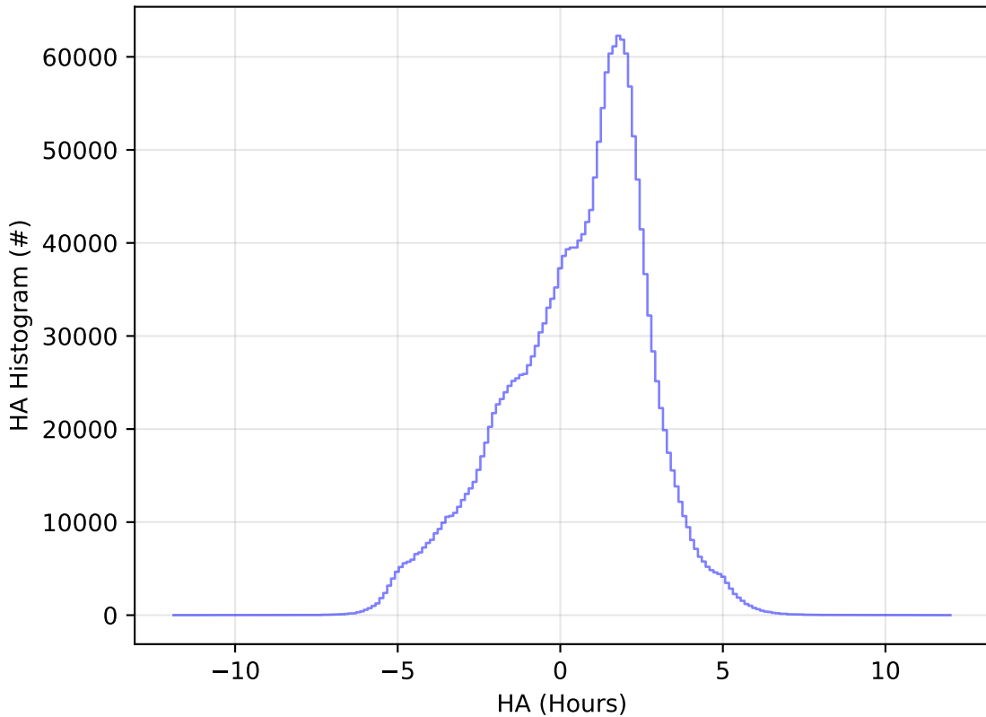
roll_uniform_early_half_mjdp253_v3.4_10yrs All sky all bands: HA Histogram
