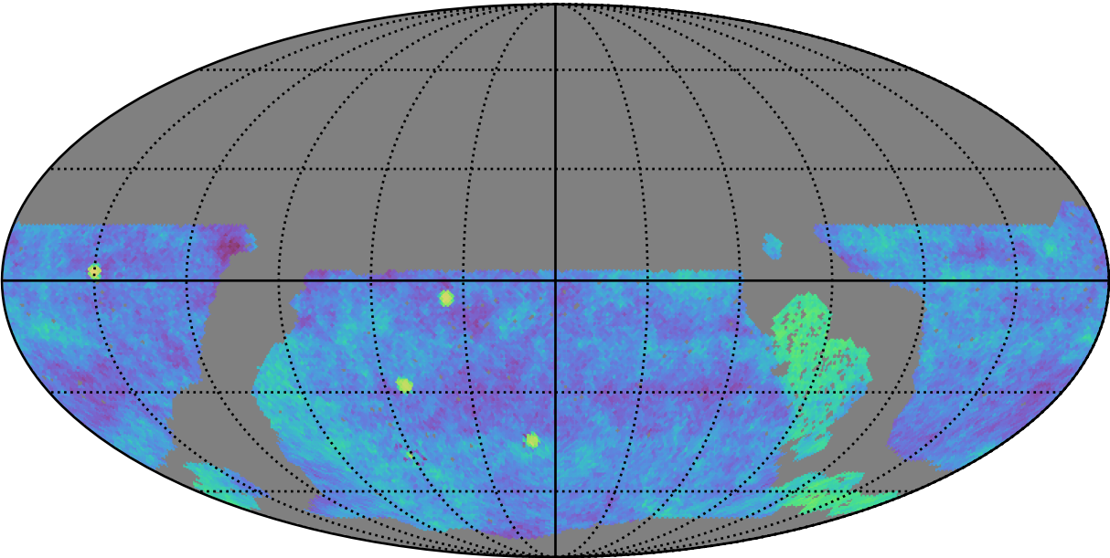
roll_uniform_early_half_mjdp253_v3.4_10yrs gri WFD: Fraction of visits in pairs (20-90 min)
