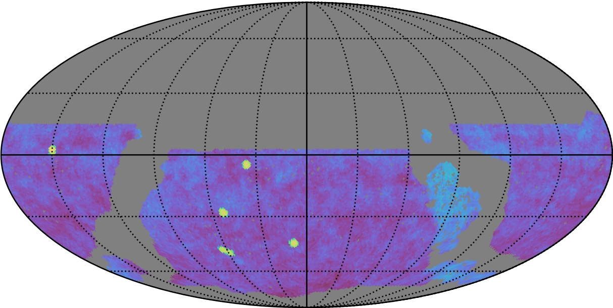
roll_uniform_early_half_mjdp253_v3.4_10yrs gri WFD: Fraction of visits in pairs (10-60 min)
