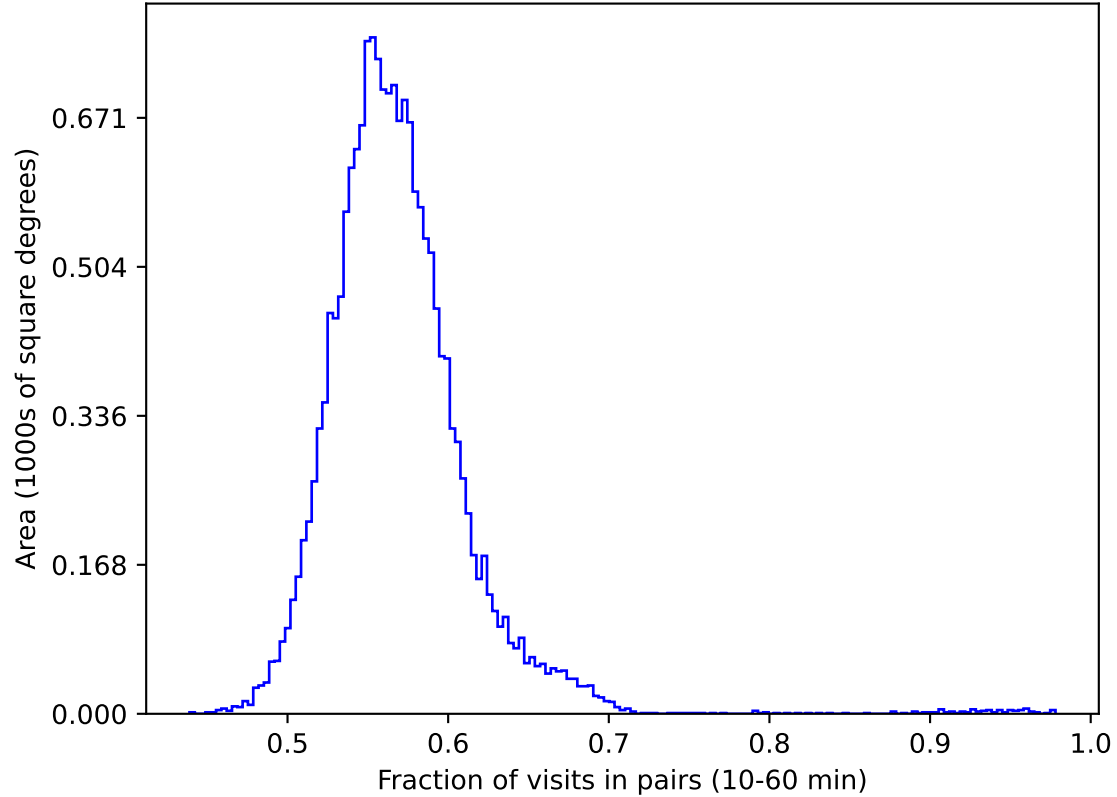
roll_uniform_early_half_mjdp253_v3.4_10yrs gri WFD: Fraction of visits in pairs (10-60 min)
