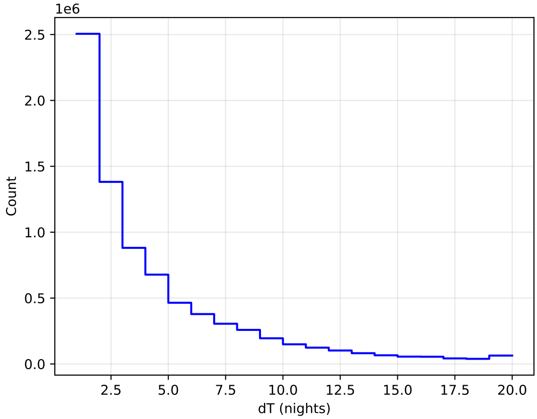
roll_uniform_early_half_mjdp253_v3.4_10yrs WFD all bands: DeltaNight Histogram
