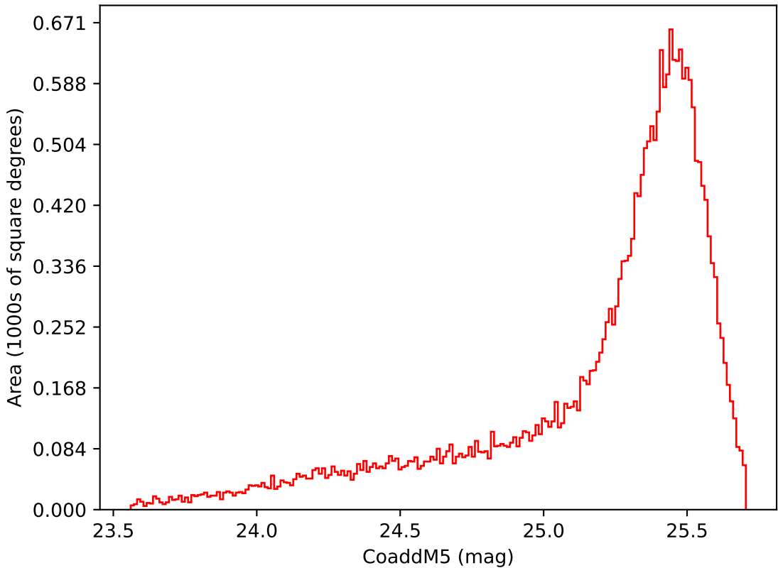
roll_uniform_early_half_mjdp253_v3.4_10yrs Yr 1 i band: CoaddM5
