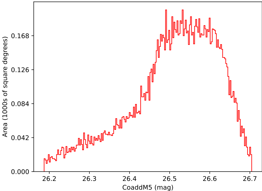
roll_uniform_early_half_mjdp253_v3.4_10yrs WFD i band: CoaddM5
