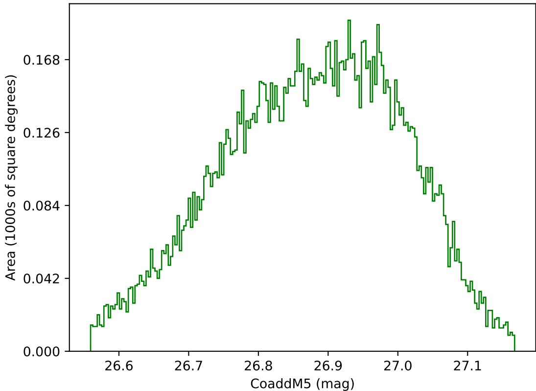
roll_uniform_early_half_mjdp253_v3.4_10yrs WFD g band: CoaddM5
