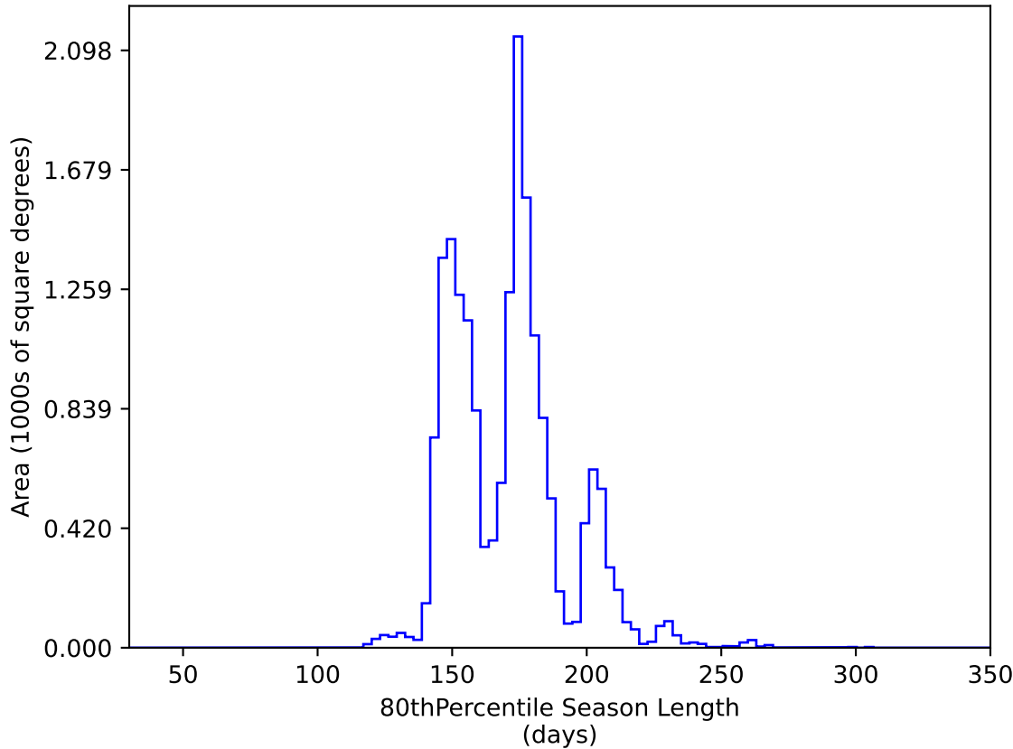
roll_uniform_early_half_mjdp253_v3.4_10yrs WFD y band: 80thPercentile Season Length
