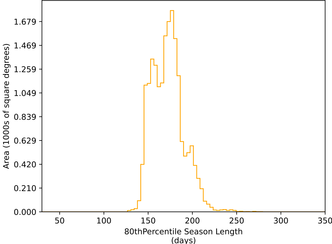
roll_uniform_early_half_mjdp253_v3.4_10yrs WFD r band: 80thPercentile Season Length
