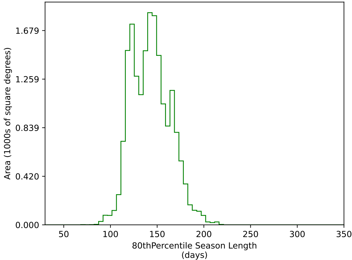
roll_uniform_early_half_mjdp253_v3.4_10yrs WFD g band: 80thPercentile Season Length
