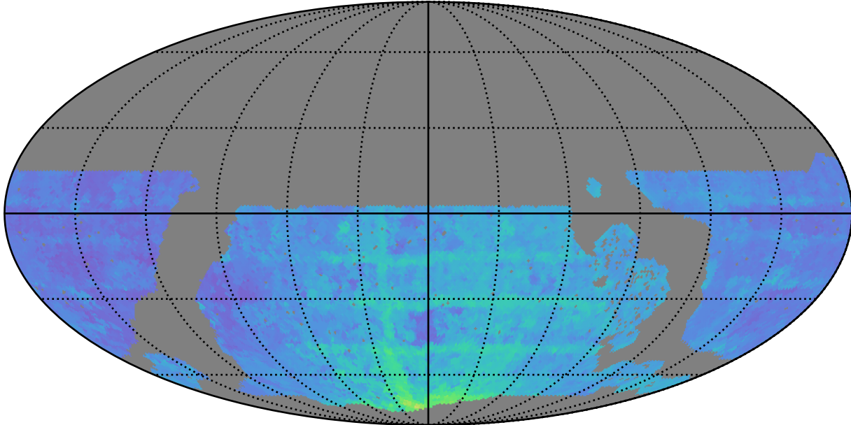
roll_uniform_early_half_mjdp253_v3.4_10yrs WFD all bands: 80thPercentile Season Length
