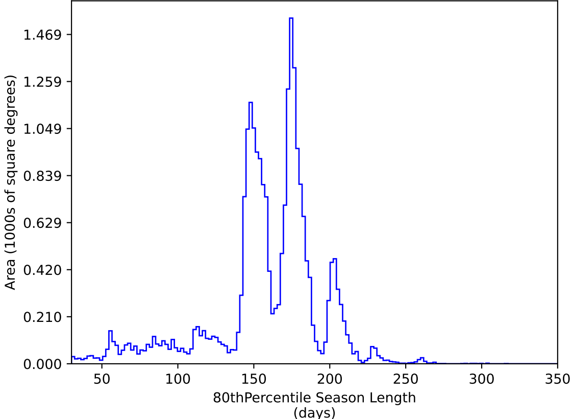
roll_uniform_early_half_mjdp253_v3.4_10yrs All sky y band: 80thPercentile Season Length
