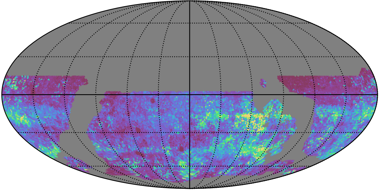
roll_uniform_early_half_mjdp253_v3.4_10yrs WFD zy bands: 75th Percentile Intranight Timespan
