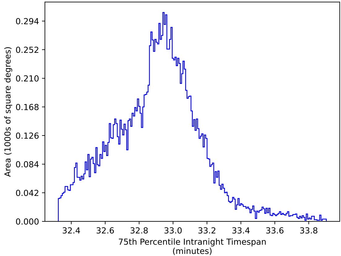
roll_uniform_early_half_mjdp253_v3.4_10yrs WFD y band: 75th Percentile Intranight Timespan
