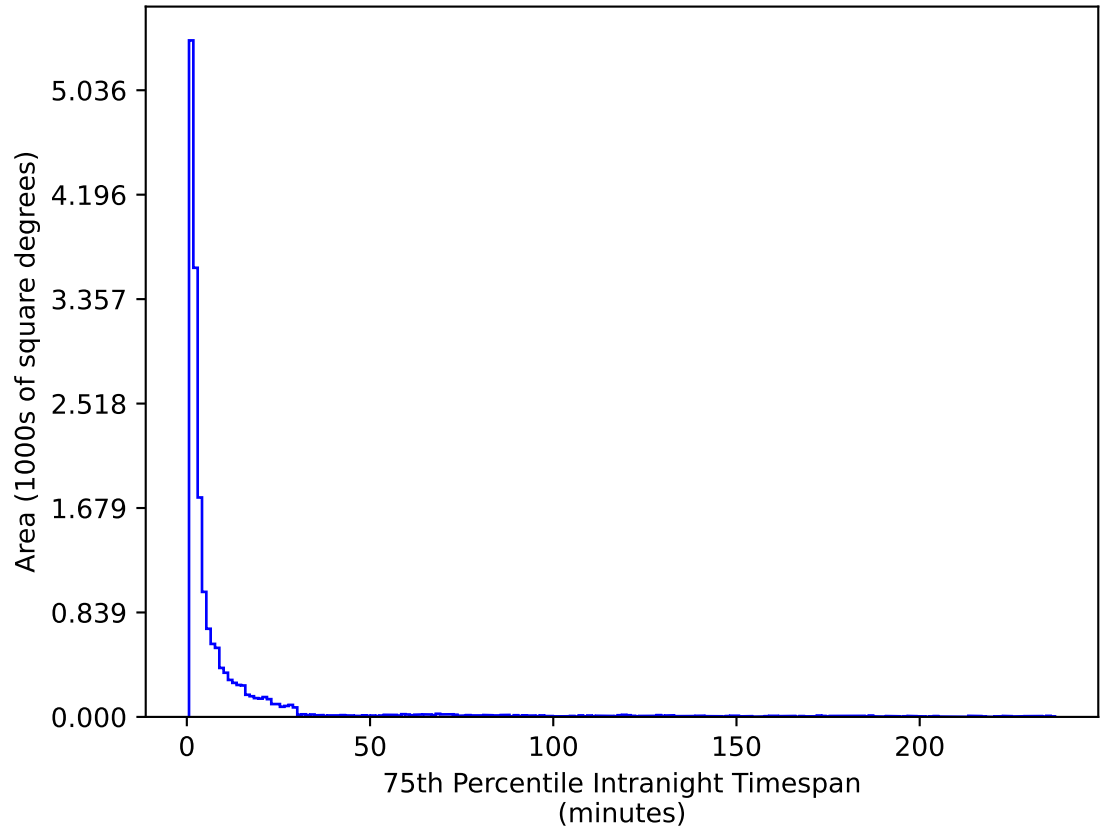
roll_uniform_early_half_mjdp253_v3.4_10yrs WFD u band: 75th Percentile Intranight Timespan
