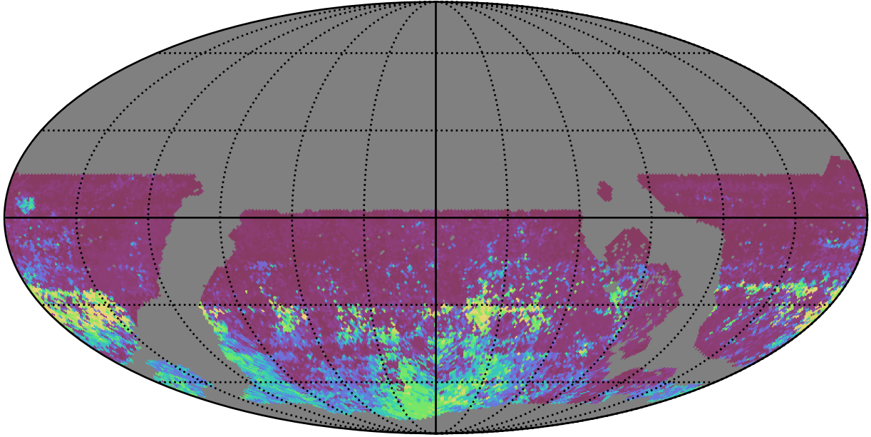
roll_uniform_early_half_mjdp253_v3.4_10yrs WFD r band: 75th Percentile Intranight Timespan
