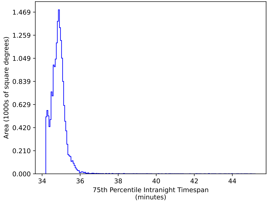
roll_uniform_early_half_mjdp253_v3.4_10yrs WFD iz bands: 75th Percentile Intranight Timespan
