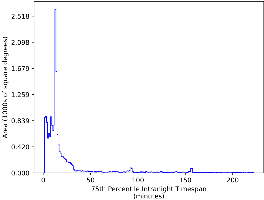
roll_uniform_early_half_mjdp253_v3.4_10yrs WFD i band: 75th Percentile Intranight Timespan
